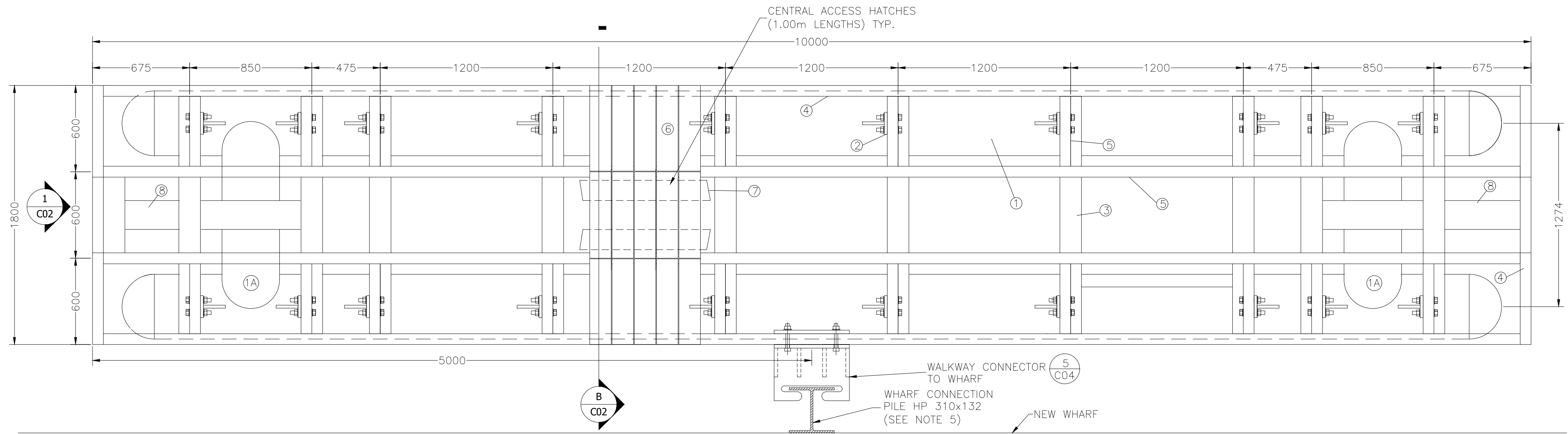
PLAN – WALKWAY (W1-10)
