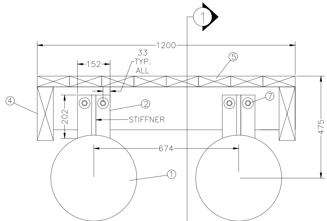
SECTION A – FINGER PIER
