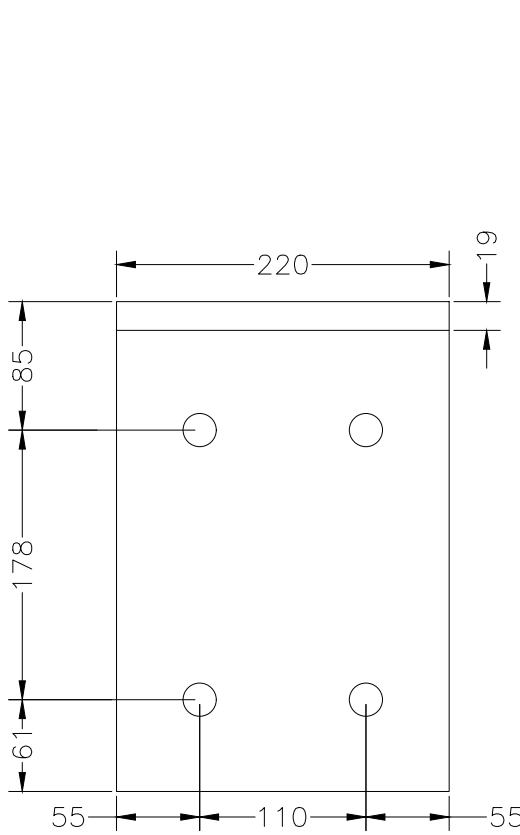
BACK VIEW
