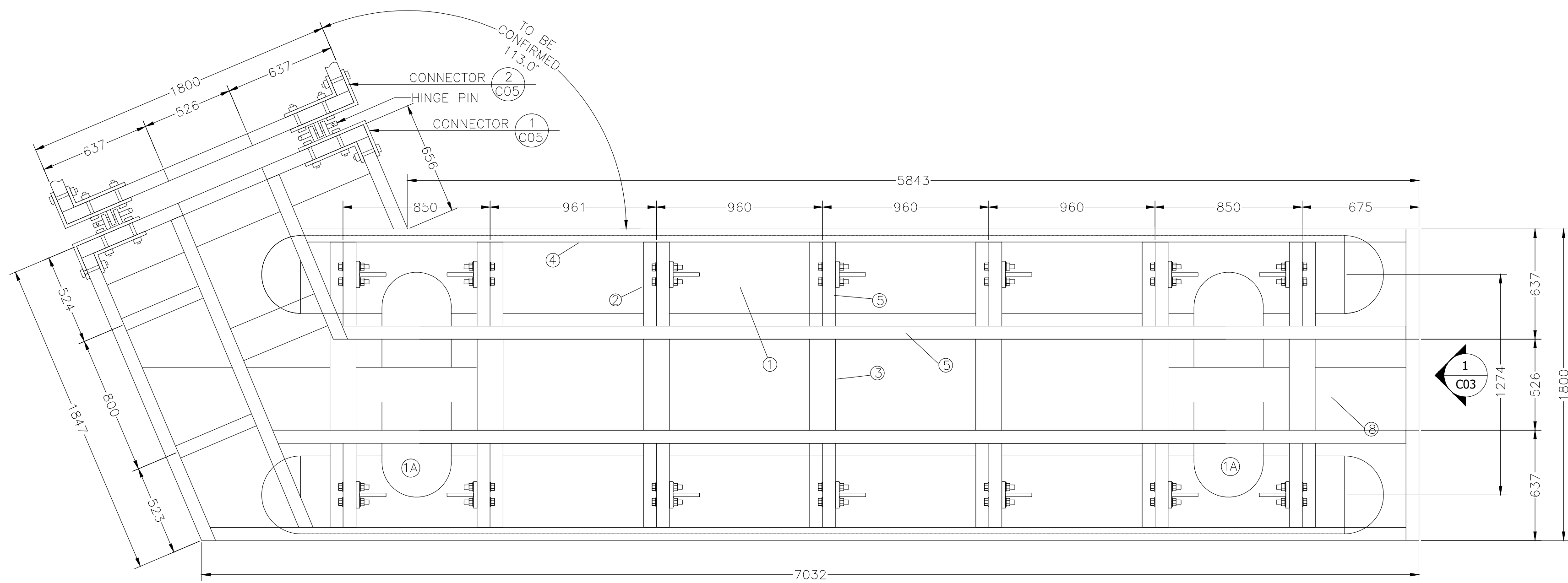
PLAN – WALKWAY (W4–8)
