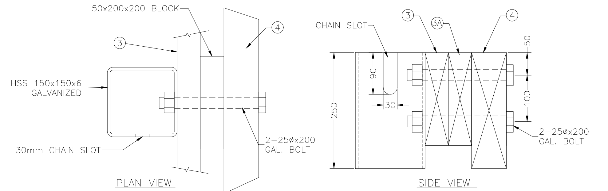
DETAIL A
