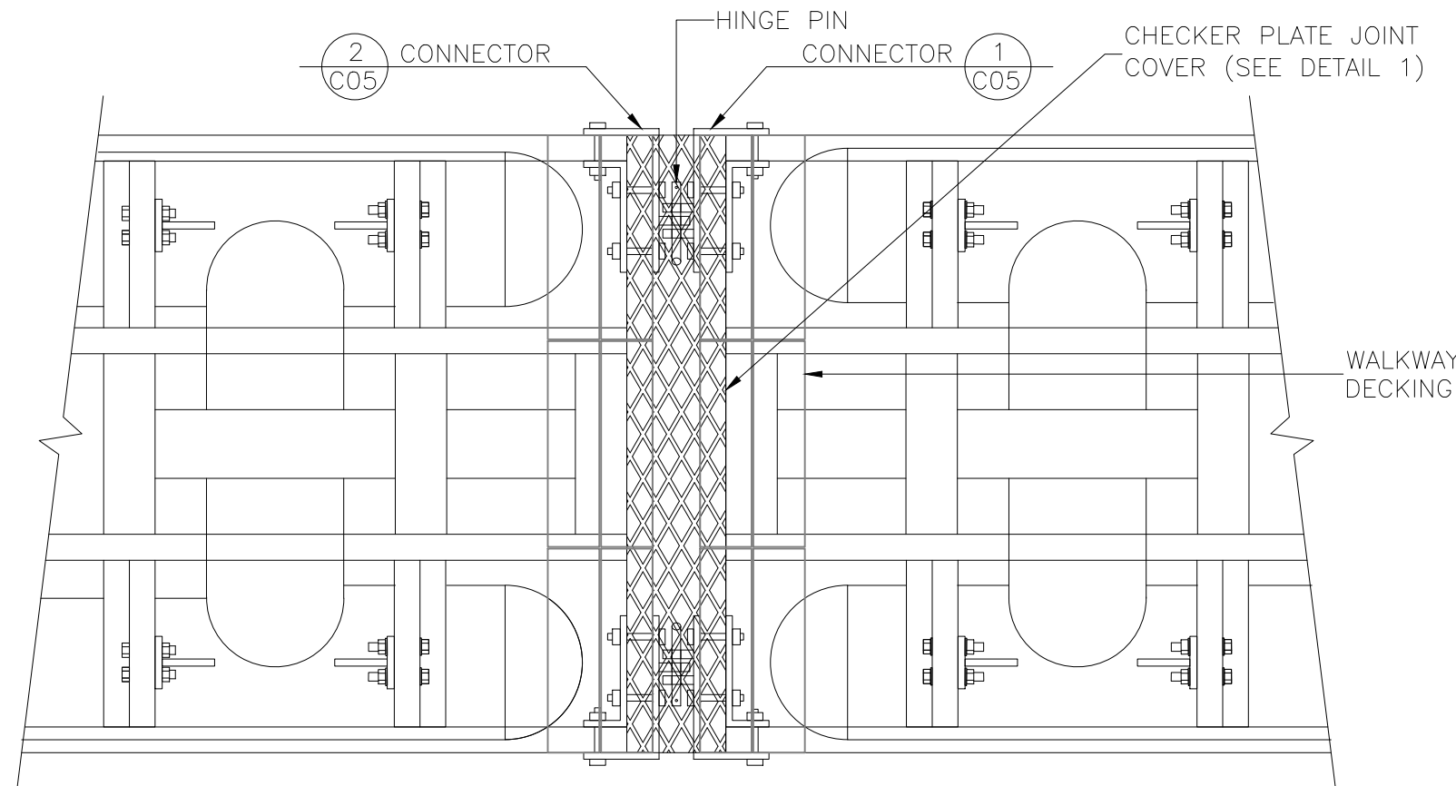
PLAN – WALKWAY CONNECTIONS (TYPICAL)
