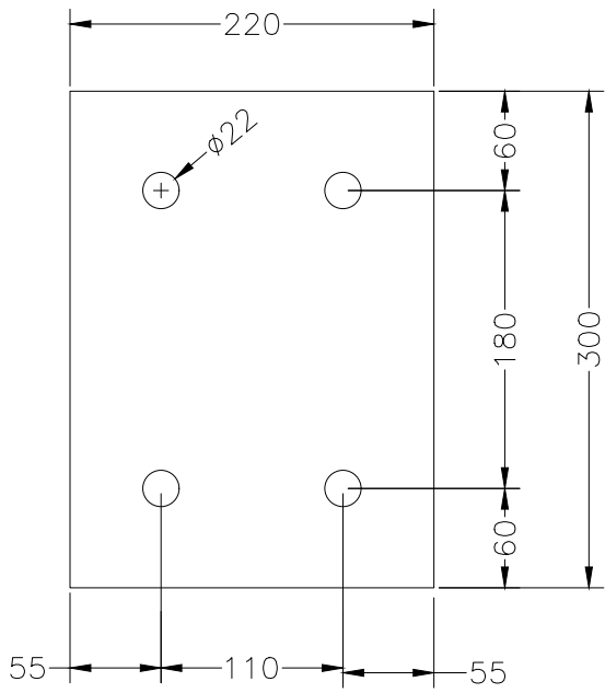
BACK VIEW
