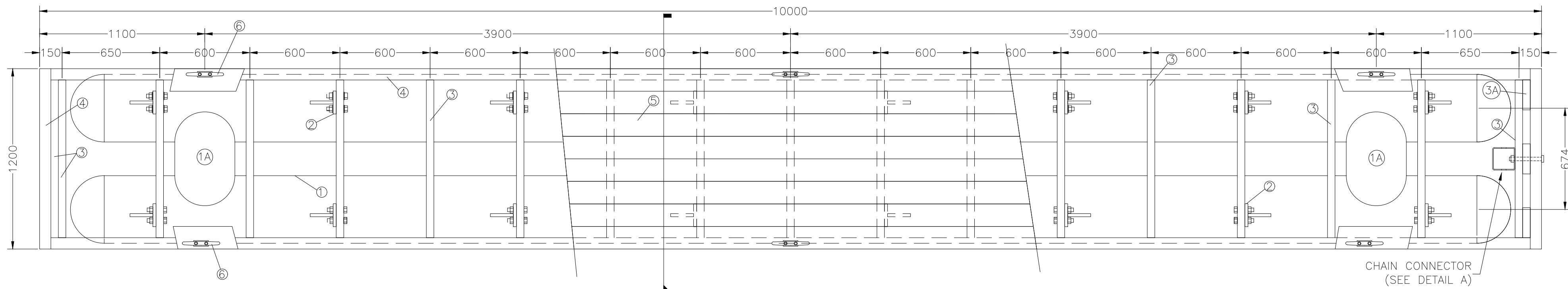
PLAN – FINGER PIER (F1)
