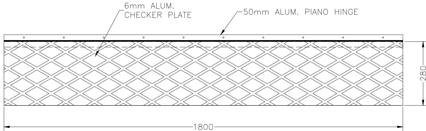
DETAIL 1
