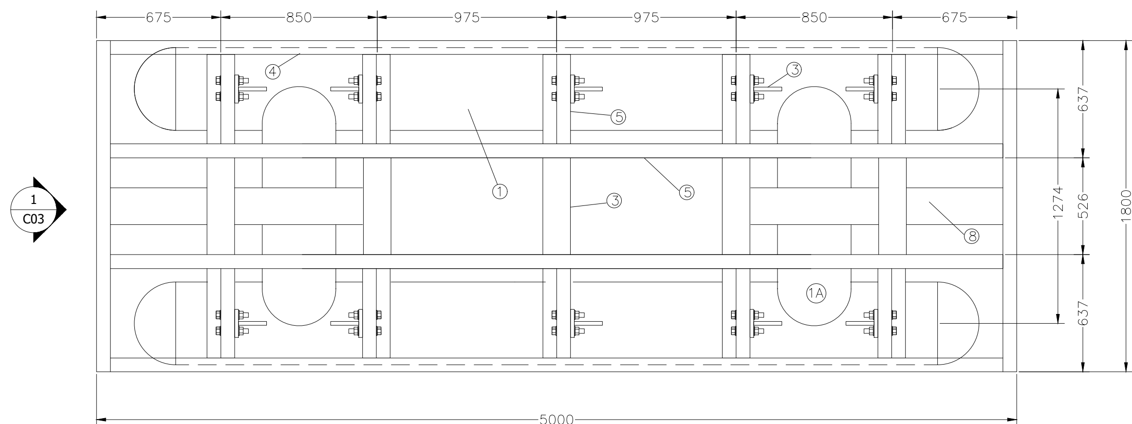
PLAN – WALKWAY (W5–5)
