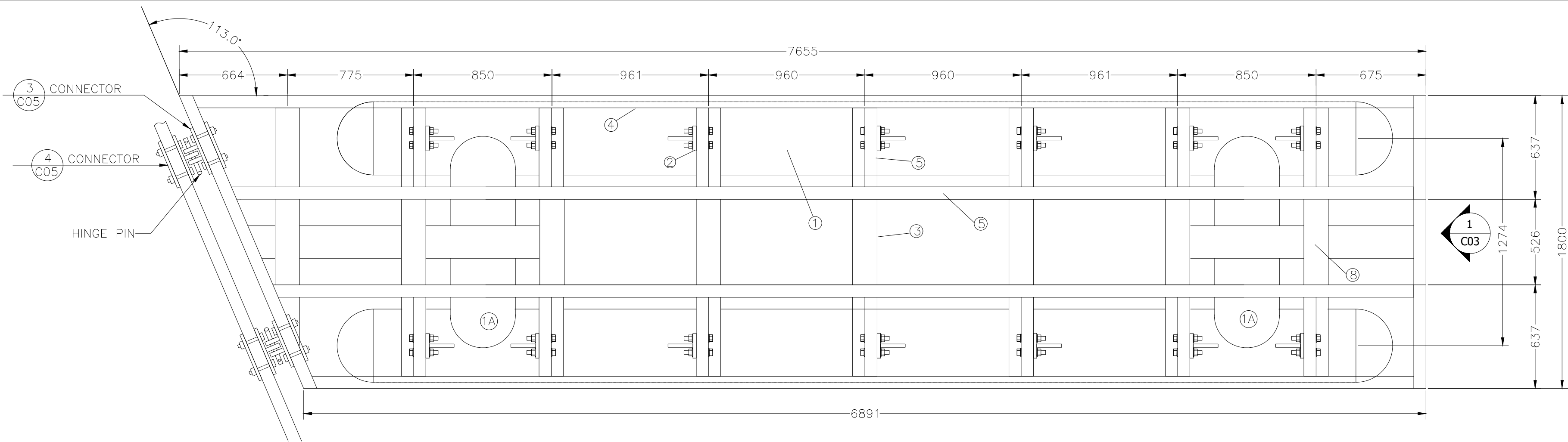
PLAN – WALKWAY (W3–7)
