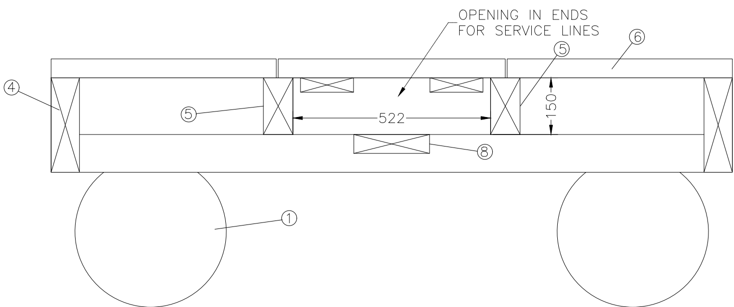
WALKWAY END VIEW
