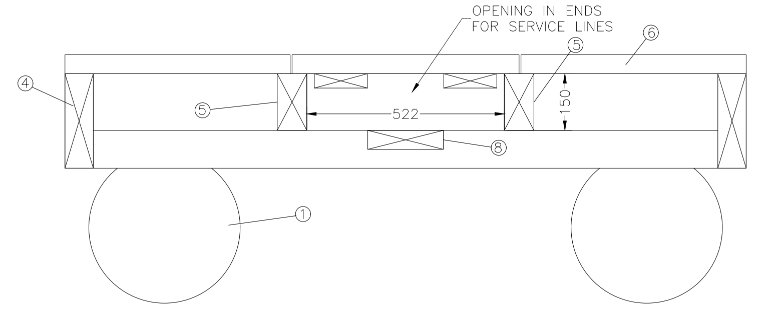
DETAIL A
